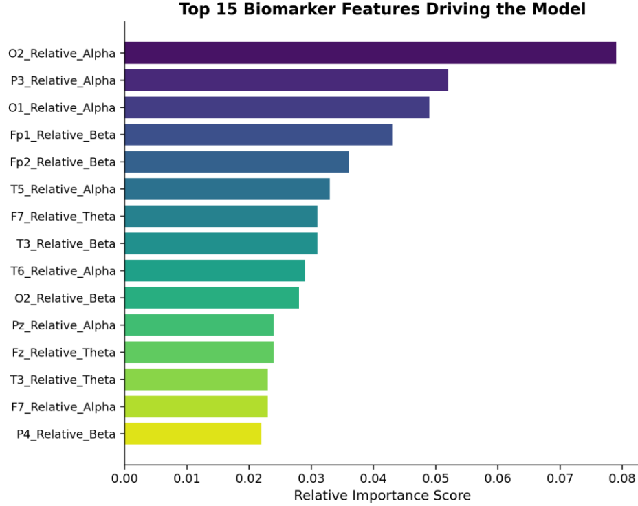
Figure 6. Top 15 features by XGBoost gain-based importance, production model (70 training subjects).
