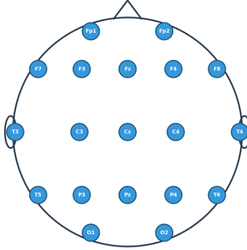
19-Channel 10-20 Montage Used for Feature Extraction
